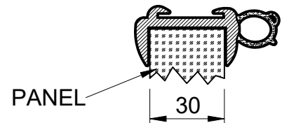
FITTED VIEW SCALE 1:2
